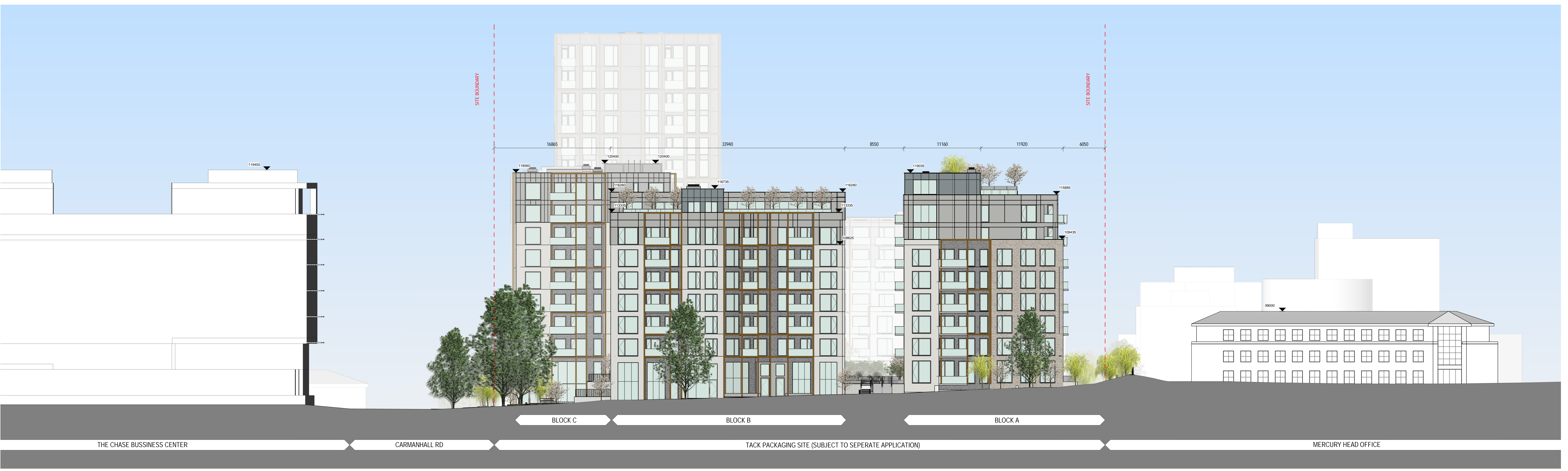
2 PROPOSED MASTERPLAN NORTH WEST CONTEXTUAL ELEVATION Scale: 1:200
